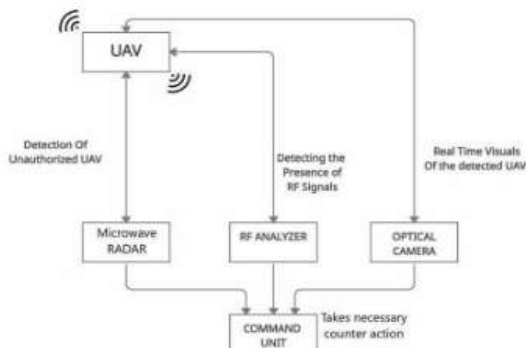
Figure 2.1: Block Diagram
