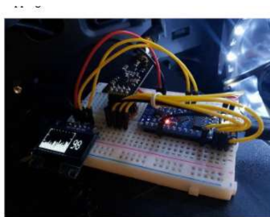
Figure 2.2: nRF24L01 transceiver designed as a RF scanner
