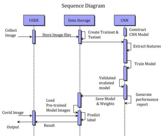
Fig. 8. Sequence diagram
