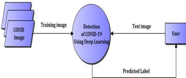
Fig. 6. Level 0 Data Flow diagram
