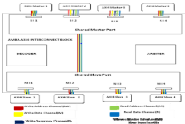
Figure 3: Block diagram of AMBA AXI4 bus interconnect.
