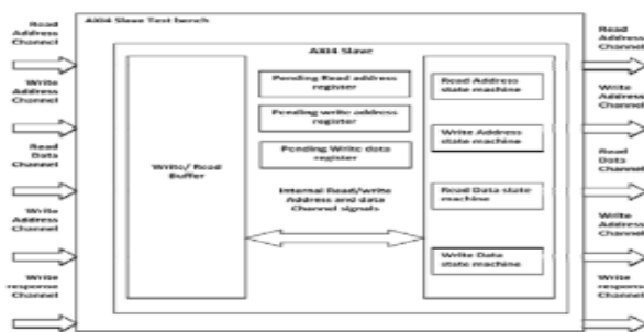
Figure 4: AMBA AXI4 slave Read/Write block Diagram.
