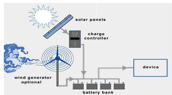
Fig. 1 Schematic of a conventional photovoltaic Hybrid System.
