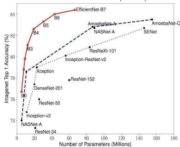
Figure 2: Efficient net performance of NetB5 architecture
