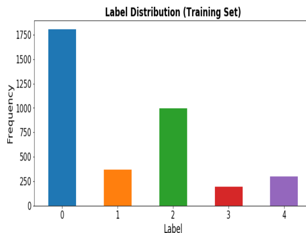
Figure 3: Label distribution
