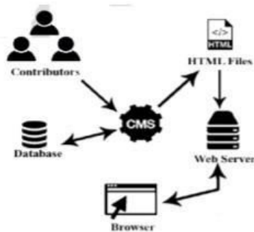
Fig.1. CMS Structure
