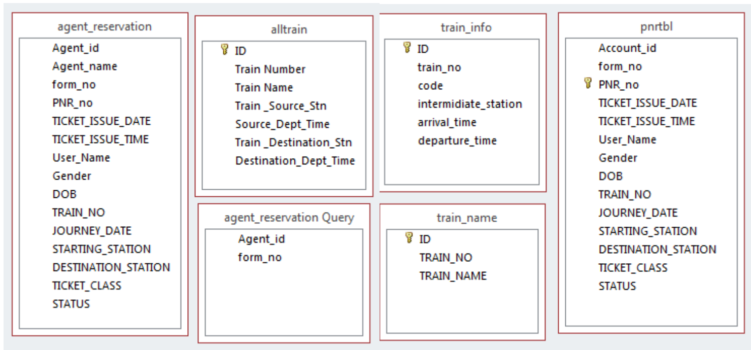
Figure 1: structure of tables in the ticket reservation database.
