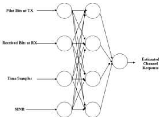
Fig.2 System Model
