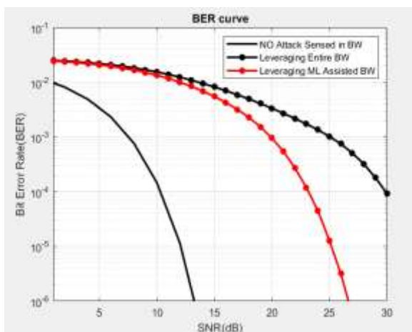
Fig.9 Error Rates for Different Conditions
