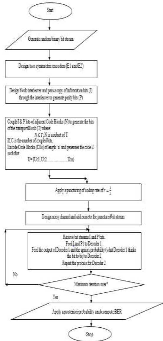
Fig.8 Proposed Flowchart
