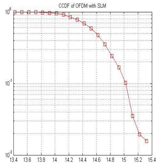
Fig.7 CCDF of Conventional SLM
