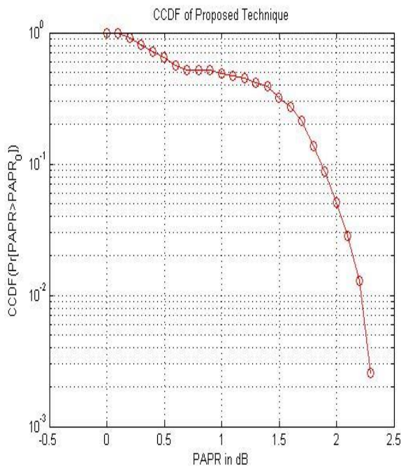
Fig.8 CCDF Proposed Technique
