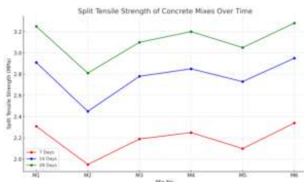
Fig 3.3.1 : Split Tensile Strength test results
