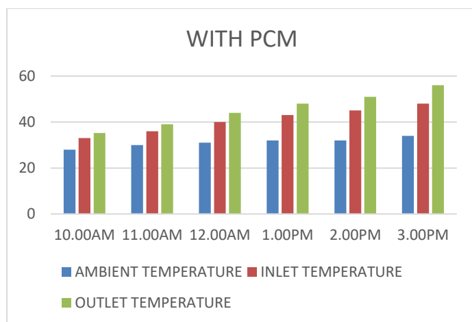
GRAPH 7.1 WITHOUT Vs WITH PCM IN SOLAR WATER HEATER
