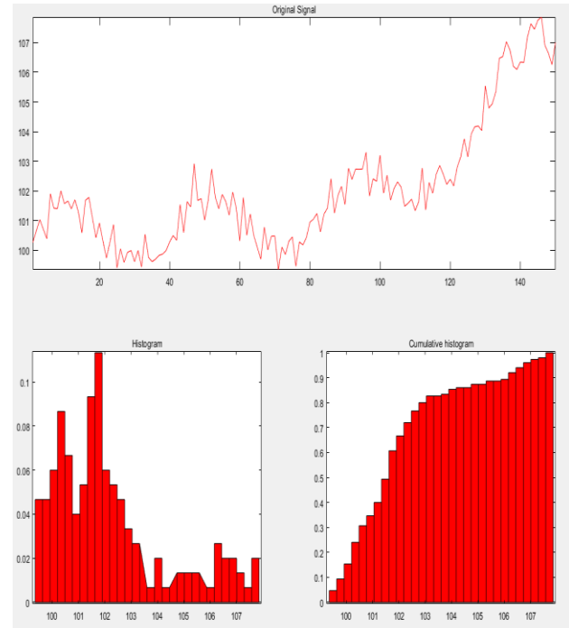
Fig. 4 Original Histogram
