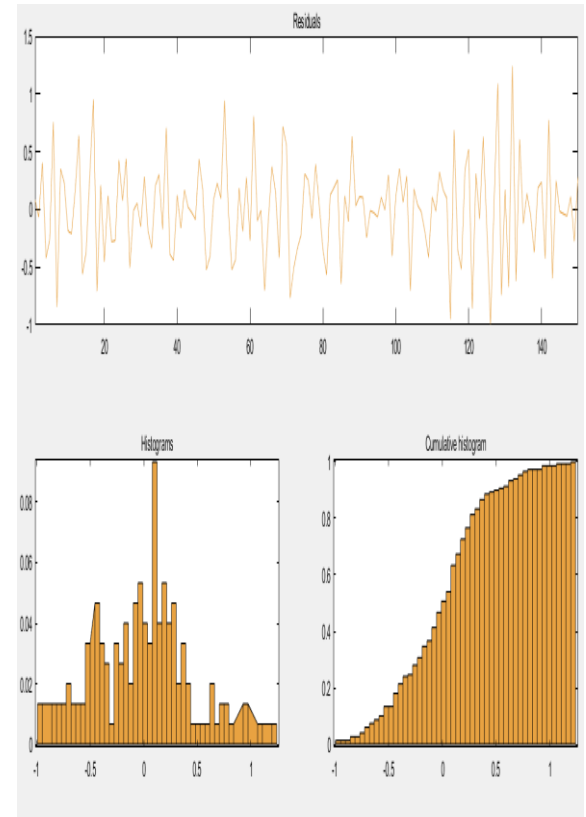
Fig. 7 Residual Histograms
