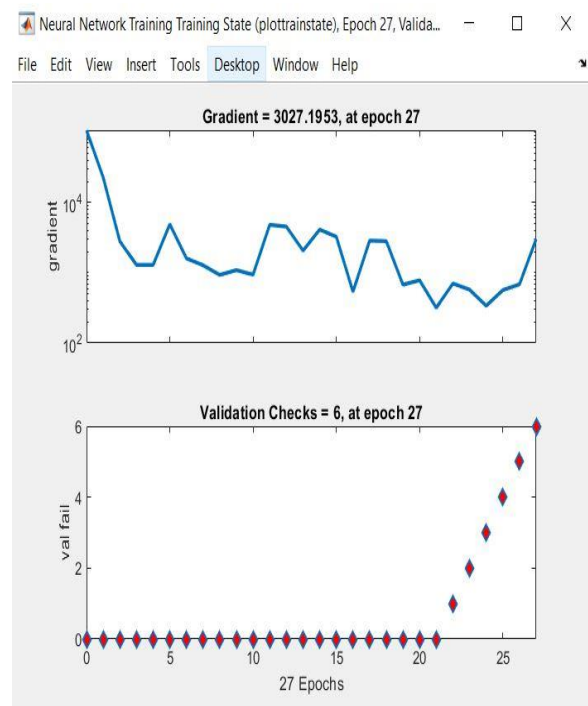
Fig.8 Training Parameters
