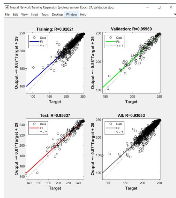
Fig.9 Regression Analysis
