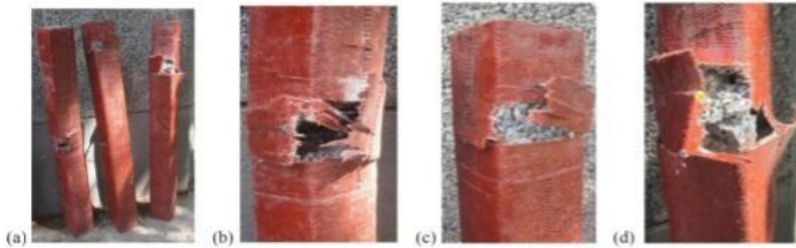
Fig. 11. Failure mode of Column S2R1.
