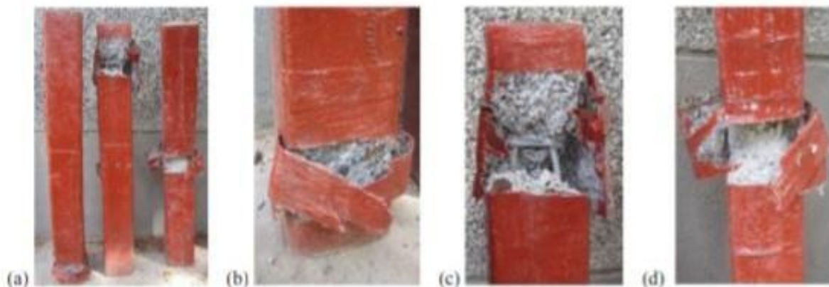
Fig. 10. Failure mode of column S1R1
