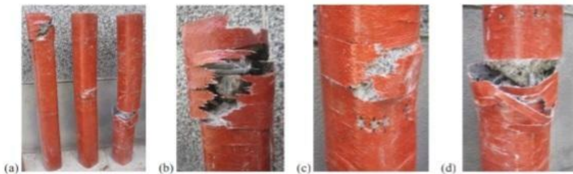
Fig. 12. Failure mode of Column S1R2.
