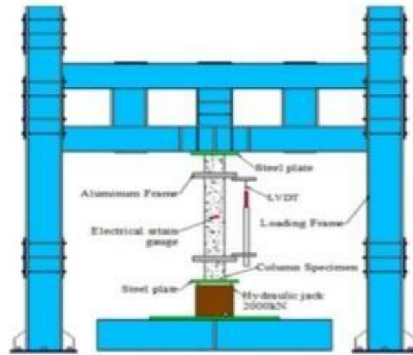
Fig. 6. Schematic view of test setup for RC column
