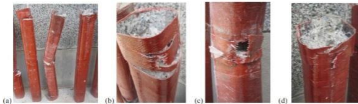
Fig. 13. Failure mode of Column S2R2.
