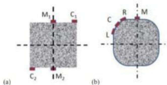
Fig. 5. (a) Strain gauges on sharp edges specimen (b) Strain gauges on corner radius specimen
