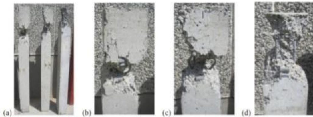
Fig. 9. Failure mode of control column S0R0
