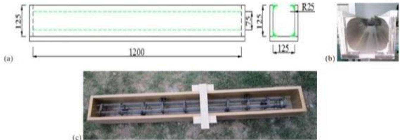
Fig. 3 (a) Schematic view of formwork for column with corner radius 25 mm, (b) Completed formwork with corner radius patty and (c) Formwork with reinforcement cage.
