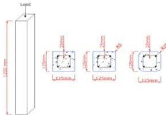
Fig. 1. RC column with different corner radii
