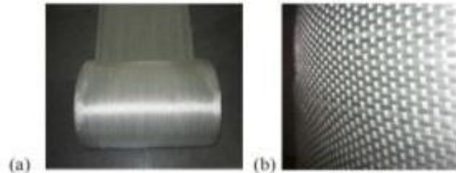
Fig. 2. GFRP Sheet (a) Sheet roll and (b) Unidirectional GFRP sheet
