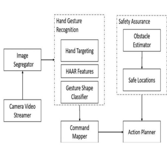
Fig. 3. Gesture Recognition and Safety Assurance System Architecture
