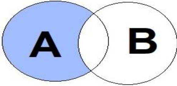
Fig.4 Probability of Exclusive Occurrence of 'A'
