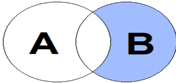
Fig.5 Probability of Exclusive Occurrence of 'B'
