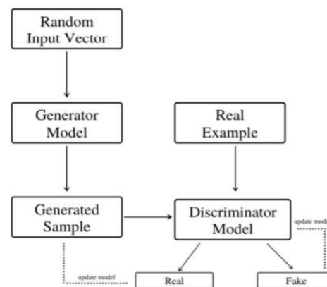
Fig. 1. A brief structure of GAN
