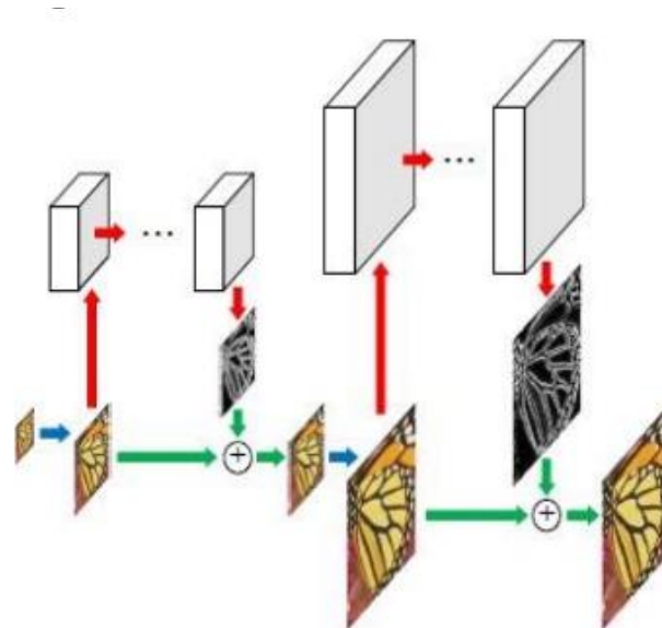
Fig. 6. Application of GAN using the Laplacian pyramid
