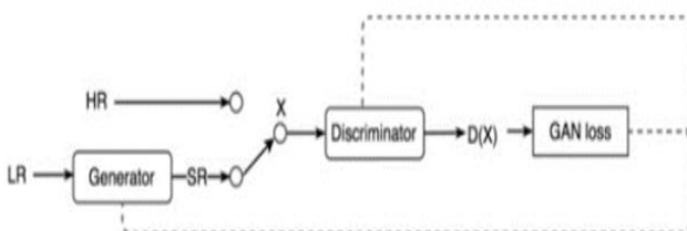
Fig. 3. Training model to implement SRGAN
