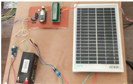
Fig. 5: Hardware implementation of the proposed method
