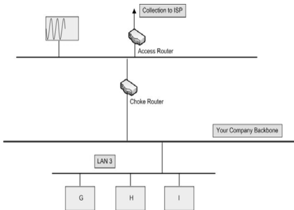
Figure 2: A sample packet filtering gateway [8]
