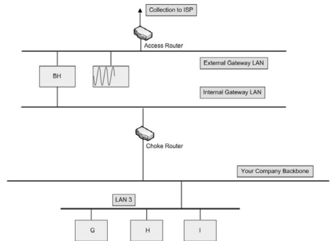
Figure 1: A sample application gateway [8]
