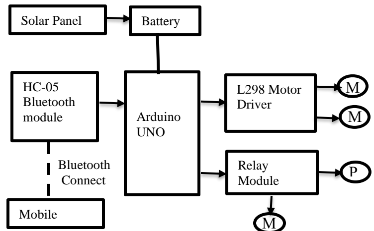
Fig.2. Block Diagram of automatic seed sowing using android app & solar panel.
