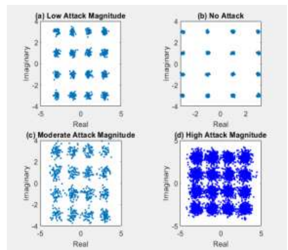
Fig.5 Scatter Plots
