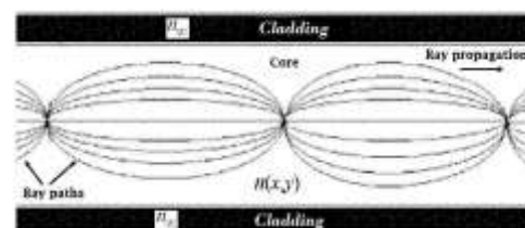
Figure 1: Light propagation in a multi-mode graded-index optical fiber (having an homogenous cladding)
