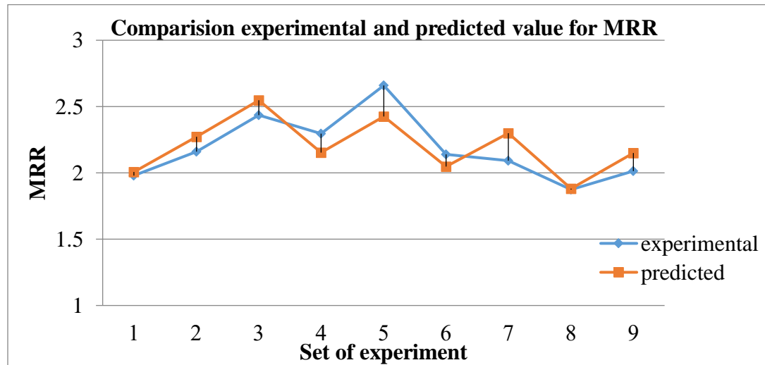
Figure 3.2 Comparison between Experimental and Predicted value of Material removal rate.
