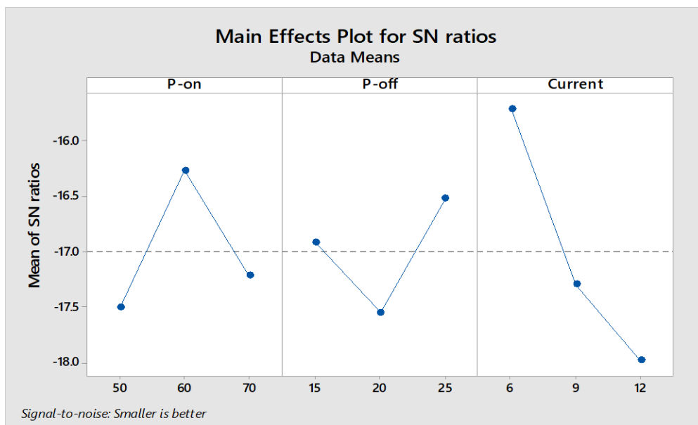
Figure.3.3 Main Effects Plot for S/N Ratio
