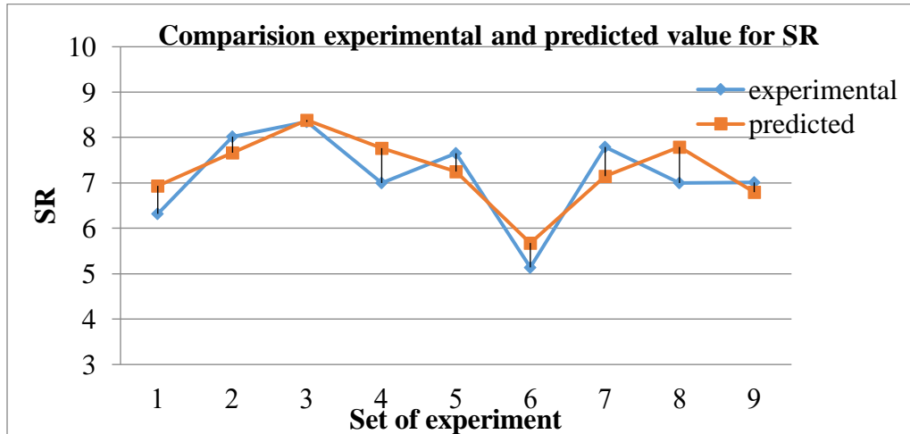
Figure 3.4 Comparison between Experimental and Predicted value of SR.
