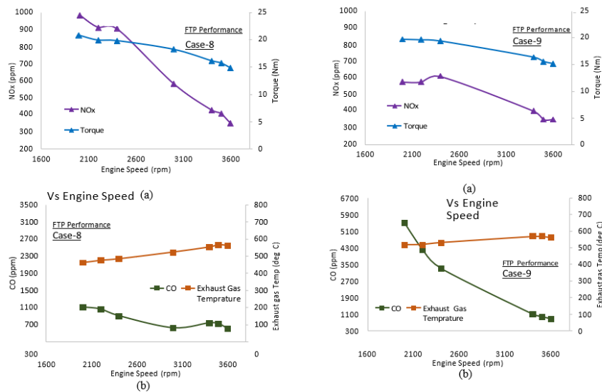
Figure 10. (a) NOx emission and engine torque vs engine speed for 9° SOI and 45° IVO; (b) CO emission and exhaust gas temperature vs engine speed for 9° SOI and 45° IVO
