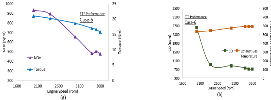
Figure 7. (a) NO x emission and engine torque vs engine speed for swirl-2 cylinder head & 45°bTDC IVO; (b) CO Figure 8. (a) NO x emission and engine torque vs engine speed for 9° SOI; (b) CO emission and exhaust gas
