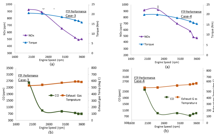
Figure 4. (a) NO x emission and engine torque vs engine speed for 30°bTDC IVO; (b) CO emission and exhaust gas temperature vs engine speed for 30°bTDC IVO
