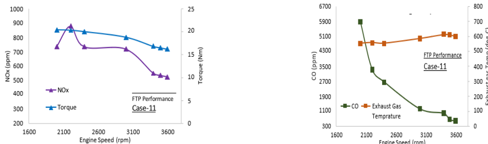
Figure 13. NOx emission and engine torque vs engine speed for 9° SOI, 45° IVO and FIP-2
