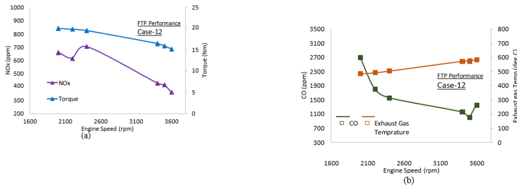
Figure 15. (a) NOx emission and engine torque vs engine speed for 7° SOI, 45° IVO, swirl-2 cylinder head, and FIP-2;
