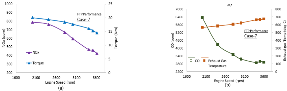
Figure 9. (a) NOx emission and engine torque vs engine speed for 7° SOI; (b) CO emission and exhaust gas temperature vs engine speed for 7° SOI
