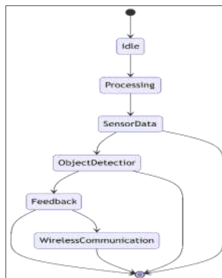
Figure 1 :System Architecture of Smart Assistive Stick for Visually Impaired People
