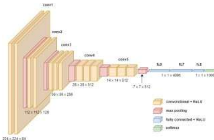
Fig 5. Stem Classification
