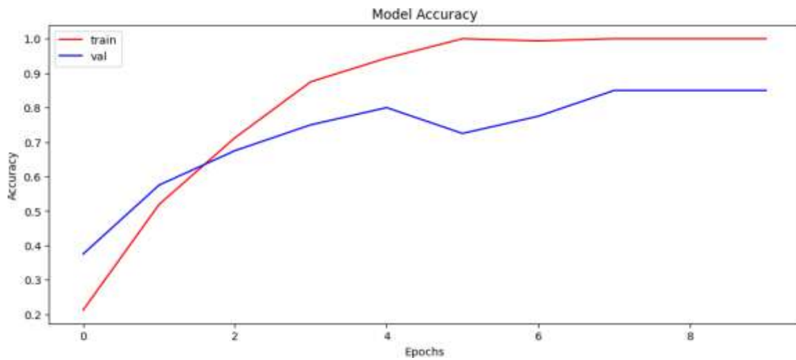
Fig 11. Model Accuracy
