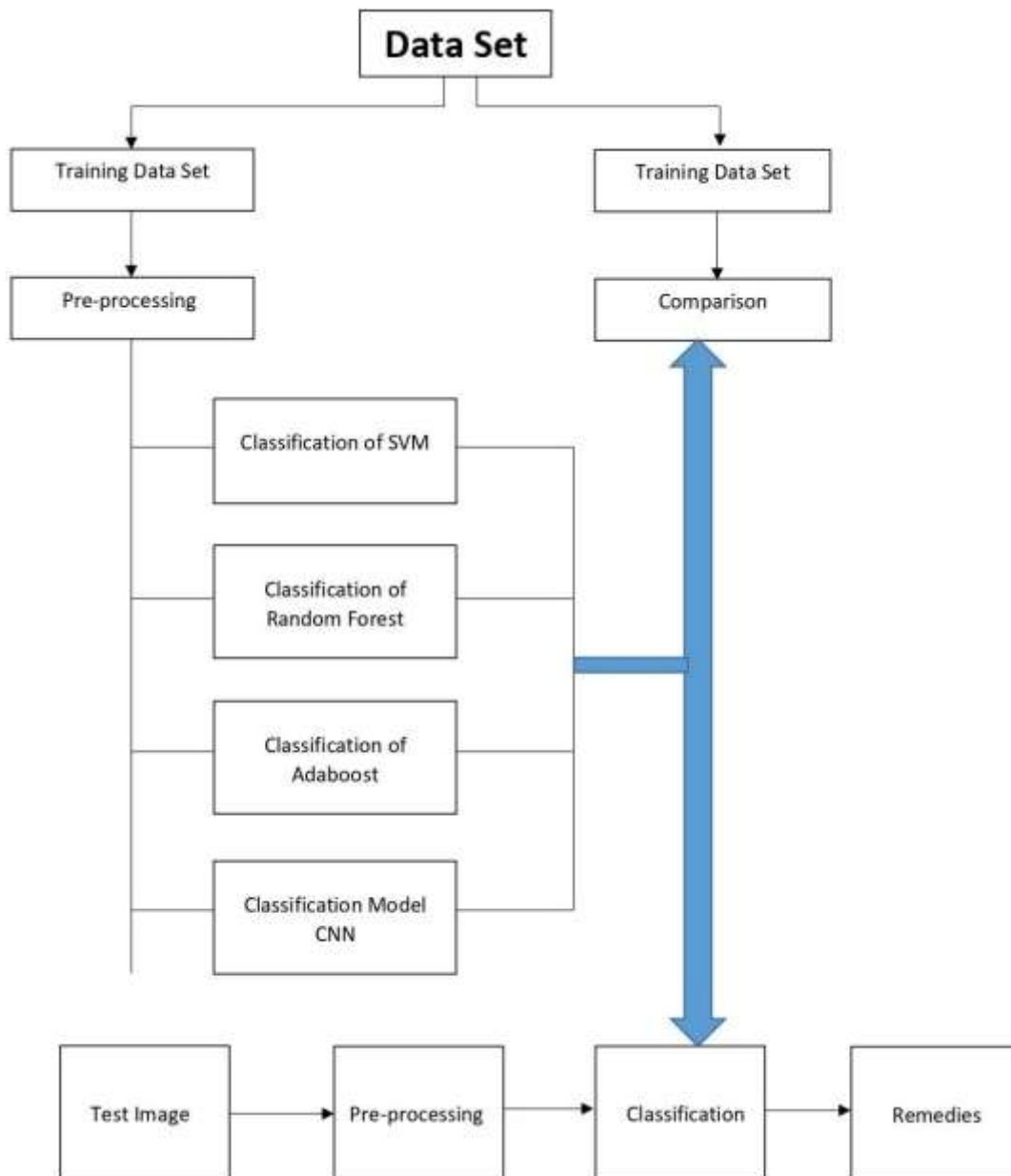
Fig 6. Process Diagram
