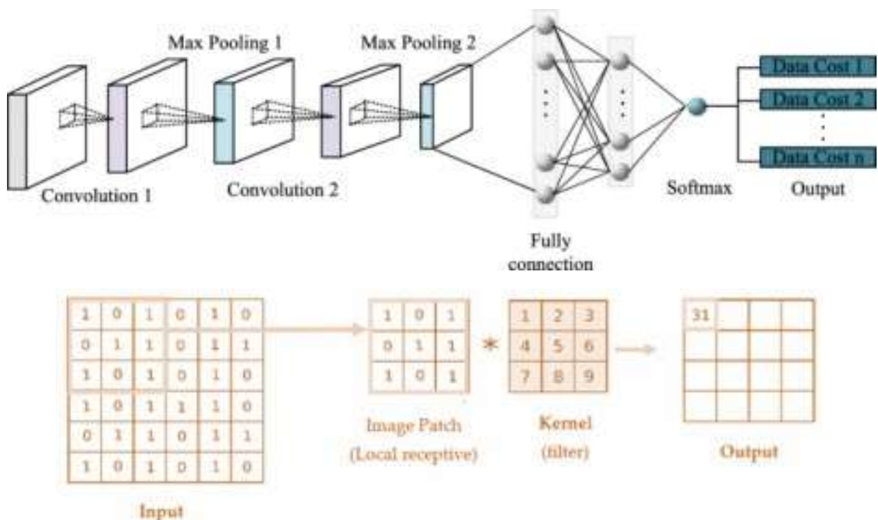
Fig 1. Convolution Layer
