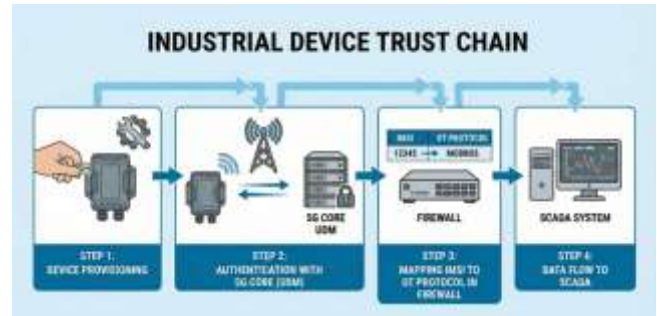
Figure 3: Onboarding and authentication of an industrial device on a private 5G network
