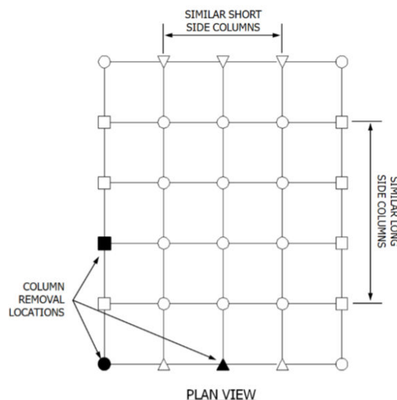
Fig 4.1 Location of External Column Removal
