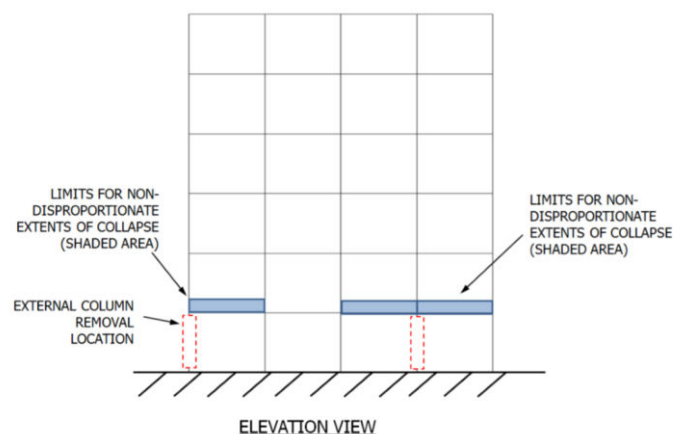
Fig 4.2 Allowable Extents of Collapse for Interior and Exterior Column Removal in Elevation
