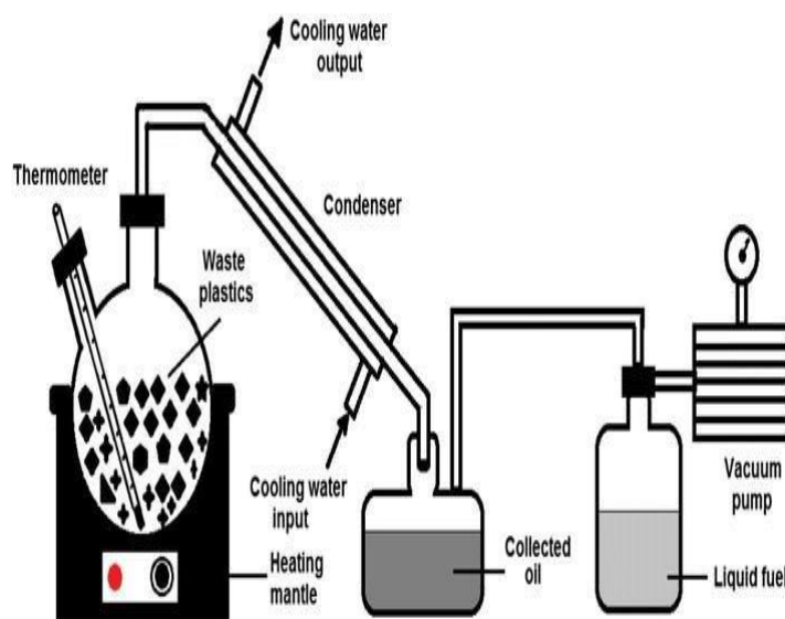
Fig. 3: Experimental Setup [3]
