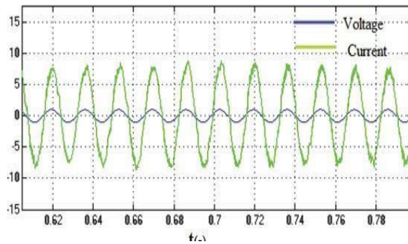
Fig.10 Power Factor Improvement Using PI Controller
