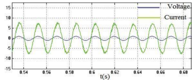
Fig.8 Phase difference between Source Voltage and Current without Compensation
