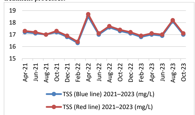
Figure 6. Total suspended solids (TSS) values of treated wastewater from the 10 MLD sewage treatment plant at Patna, Bihar (2021–2023).
