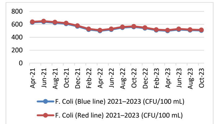
Figure 9. Fecal coliform ( F. coli ) values of treated wastewater from the 10 million liters-per-day sewage treatment plant at Patna, Bihar (2021–2023).
