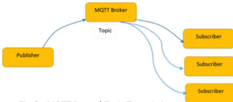
Fig. 2 MQTT Protocol Topic Transmission
