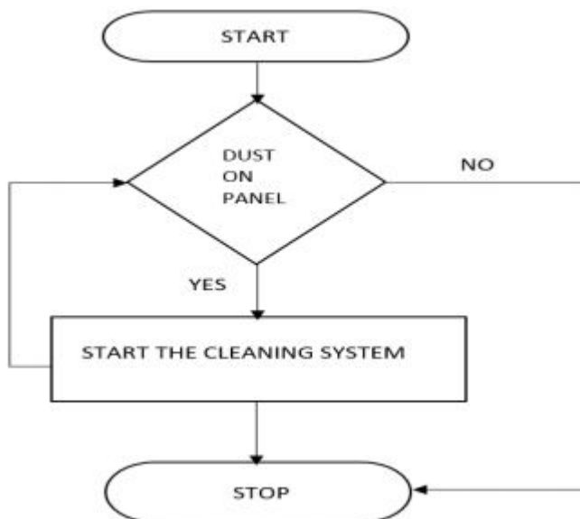
Fig.2 Automated Solar panel cleaning Algorithm.
