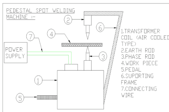
Fig..2 constructional arrangement
