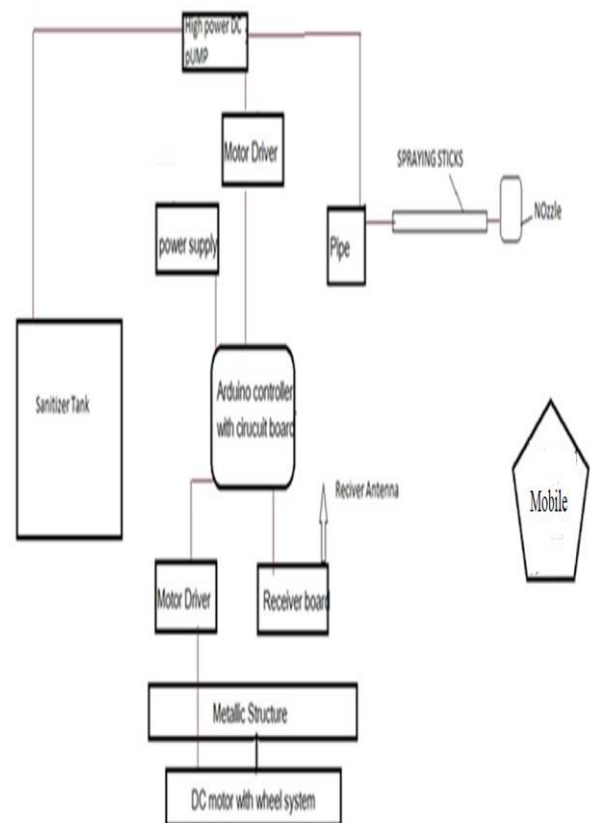
Fig. 1. Block Diagram
