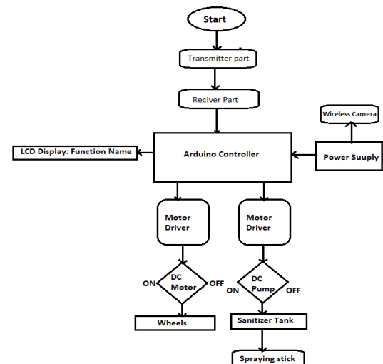
Fig.3. System flow diagram
