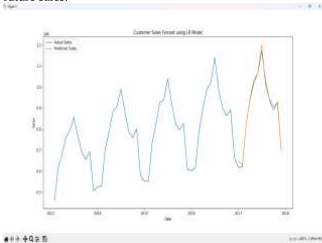
Figure 3 shows the forecasted sales generated by the machine learning model. The predicted sales closely align with the historical trends, especially during the seasonal peaks, indicating the model's ability to capture underlying patterns in customer behaviour. This is a testament to the strength of the machine learning approach in forecasting future sales.
