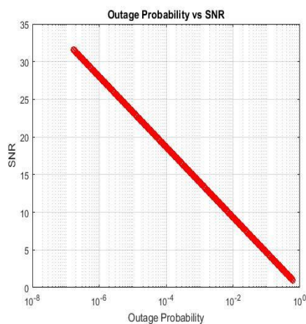
Fig. 7 Decrease in Outage with Increase in SNR
