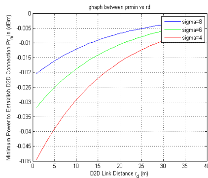
Fig. 6 Minimum Power Required to establish D2D link as a function of distance and fading (sigma)
