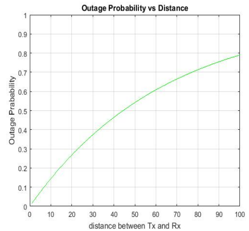
Fig. 8. Increase in Outage with Increase in Distance between Tx and Rx
