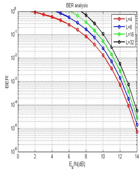
Fig. 9. BER performance of system
