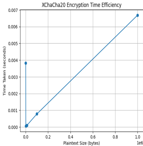
Fig 3: Xchacha20 Encryption Time Efficiency
