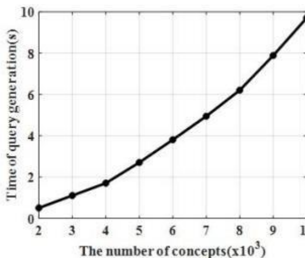
Fig 3: Time of query generation
