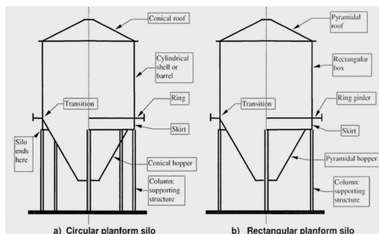
Figure 1: Terminology used in solid storage structure structures
