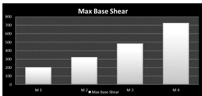
Figure 2: maximum base shear in z direction for zone V
