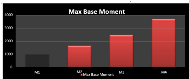
Figure 3: maximum base moment in x direction for zone V
