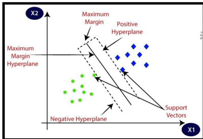
fig-4: SVM Algorithm
