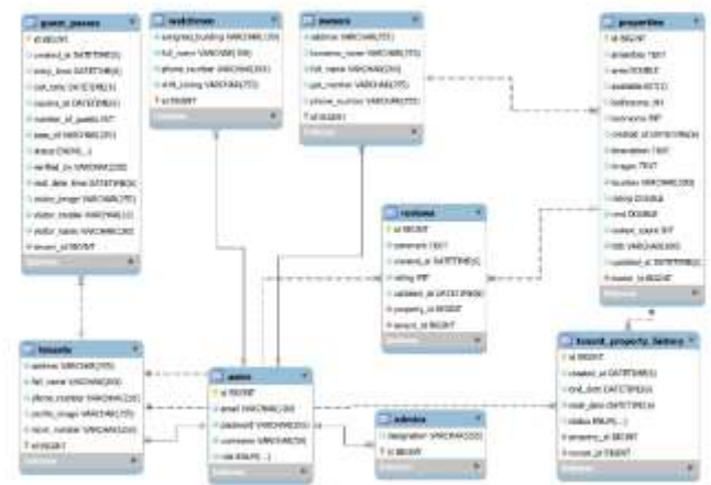
Figure 3.2.1 ER Diagram
