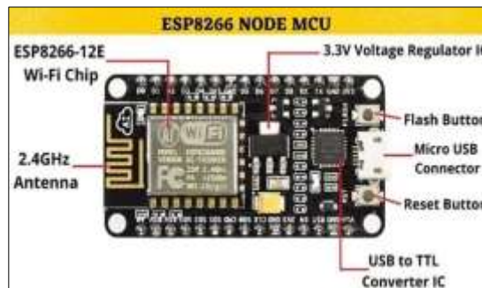
Figure 2 NODE MCU ESP8266
