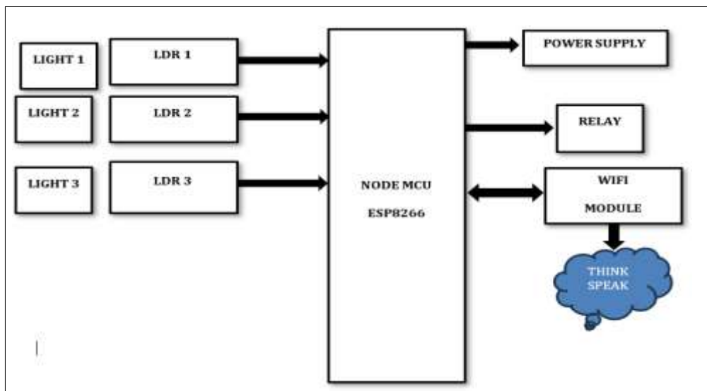
Figure 1 Block diagram
