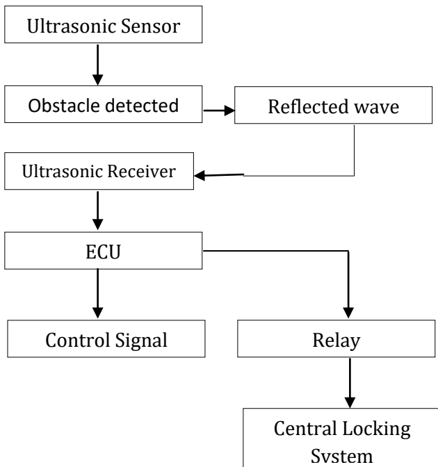
Fig 2. Block Diagram of Automated door lock system
