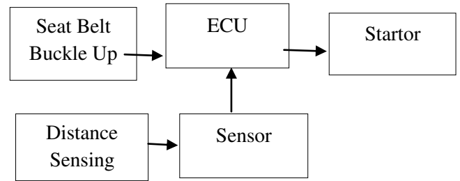
Fig 2. Block Diagram of Seatbelt alert system with ignition control
