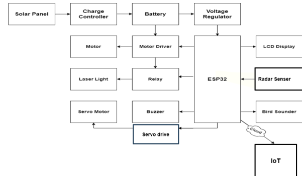
Figure 1: Block Diagram
