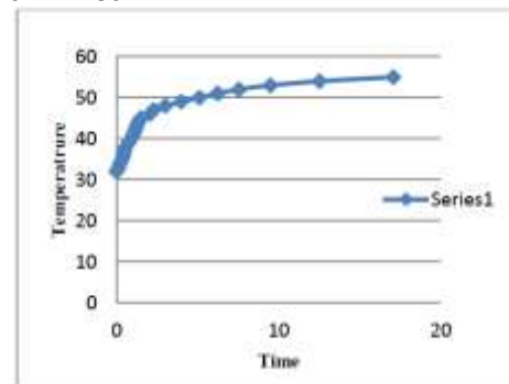
GRAPH 2-HEATING (WITHOUT LOAD)
