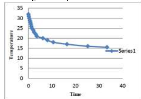
GRAPH 1-COOLING (WITHOUT LOAD)
