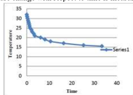
GRAPH 1-COOLING (WITHOUT LOAD)
