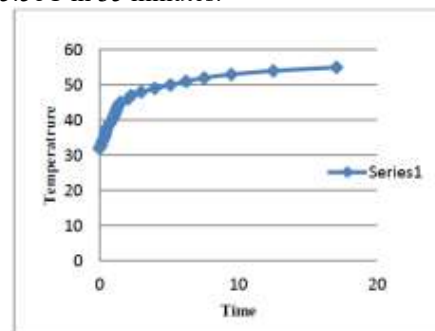
GRAPH 2-HEATING (WITHOUT LOAD)
