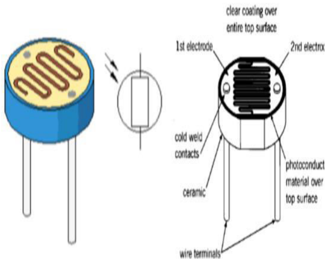
Fig 2. Light Dependent Resistor
