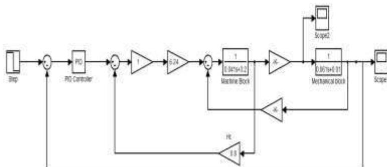
Figure10.SIMULINK Block Diagram of a Closed Loop PMSM Drive Using PI Current Controller and PID Speed Controller
