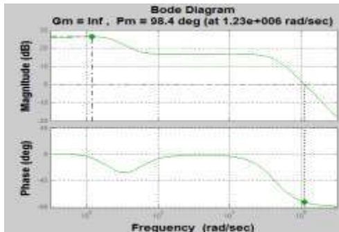
Figure27. Bode Diagram Representation of Overall Speed and Current Loop Both Using PID Controller
