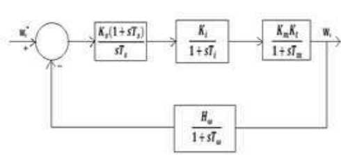
Figure6.SimplifiedSpeedControlLoop
