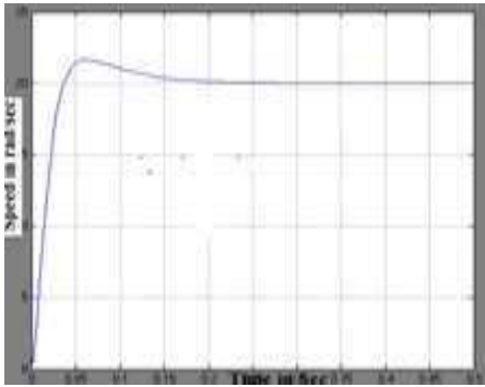
Figure17. Actual Speed vs. Time Wave for m using P Current Controller and PI Speed Controller of the Closed Loop Adjustable Speed PMSM Drive When a Step Change in Reference Speed of 20 rad/sec is introduced
