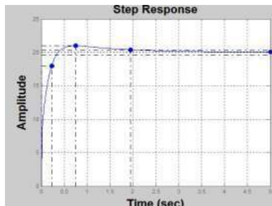
Figure26.Step Response Characteristics of Overall Speed and Current Loop Both Using PID Controller
