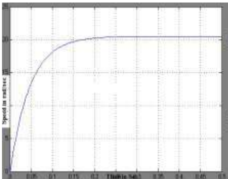
Figure21. Actual Speed vs. Time Waveform Using PI Current Controller and PID Speed Controller of the Closed Loop Adjustable Speed PMSM Drive When a Step Change in Reference Speed Of 20 Rad/Sec Is Introduced
