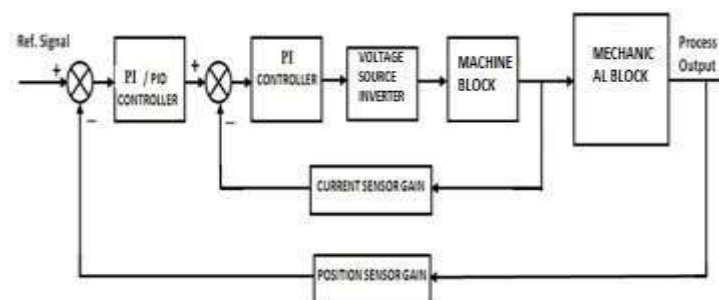
Figure 3. Systematic Block Diagram Representation of a Closed Loop Adjustable Speed PMSM Drive The reset time and gain of
