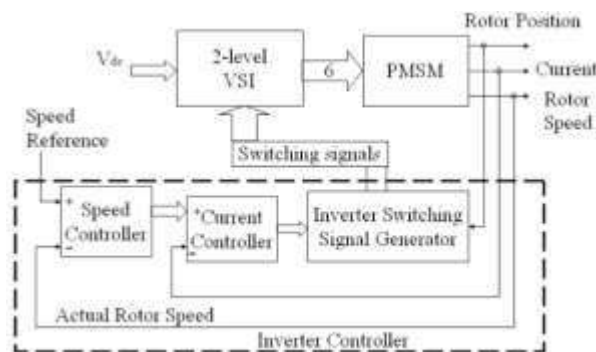
Figure1.Schematic Block Diagram of Closed Loop Model of Adjustable Speed PMSM Drive
