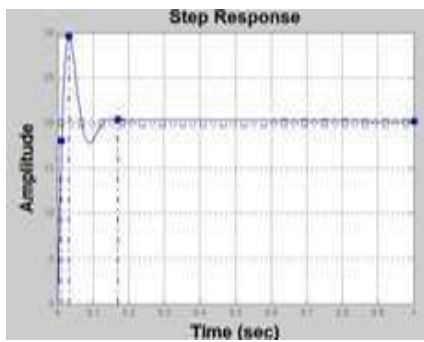
Figure13. Step Response Representation of Simplified Speed Control Loop with PID Controller
