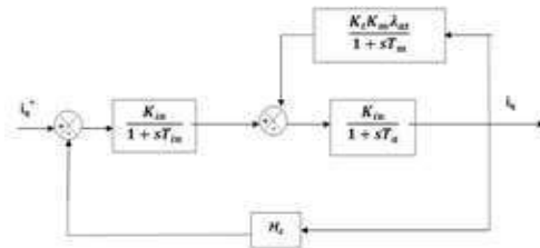
Figure5.CurrentControl Loop
