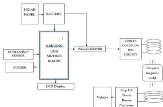
Figure1: System Design
